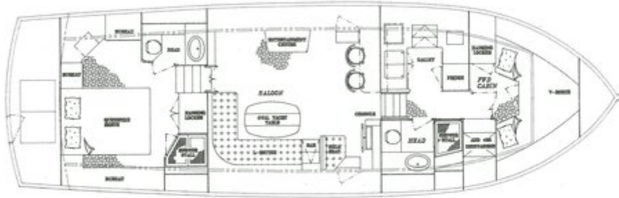
GB 46CL ARRANGEMENT PLAN 46#102
