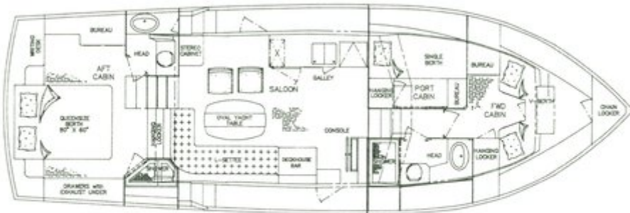
GB42 M/YACHT ARRANGEMENT PLAN
